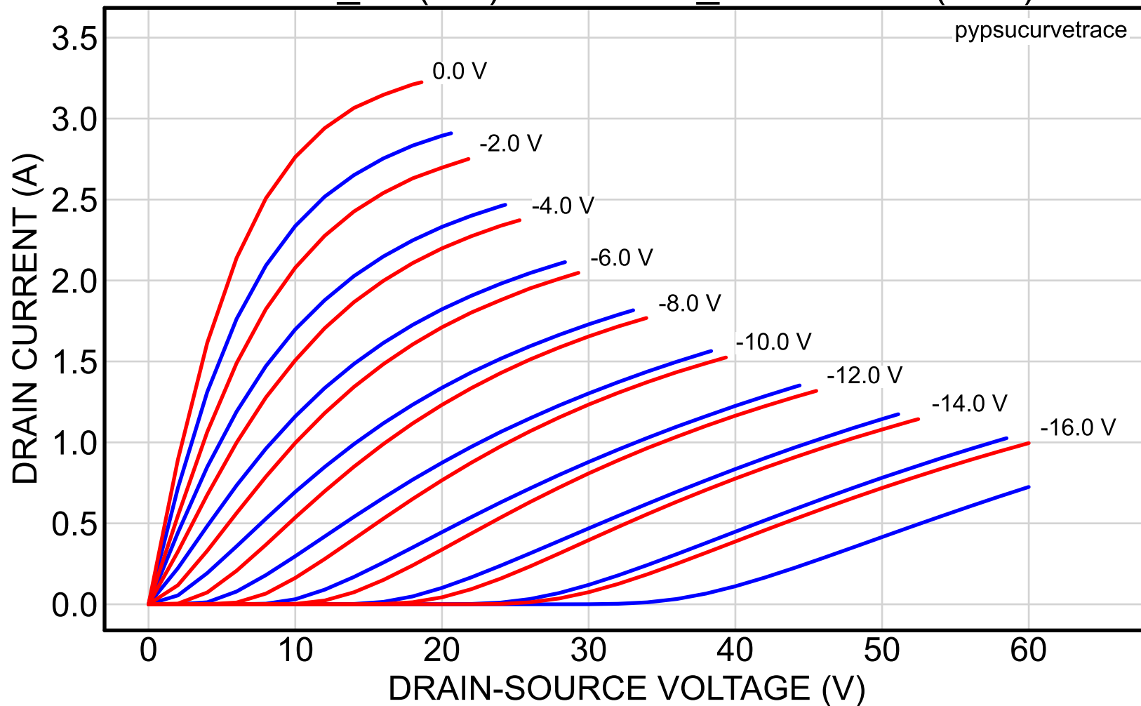
2SK82_46 (red) vs. 2SK82_56reserved (blue)
