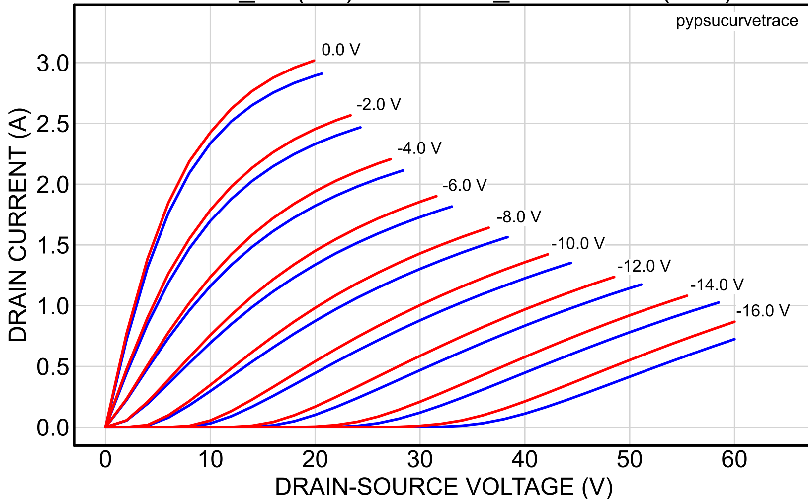
2SK82_47 (red) vs. 2SK82_56reserved (blue)
