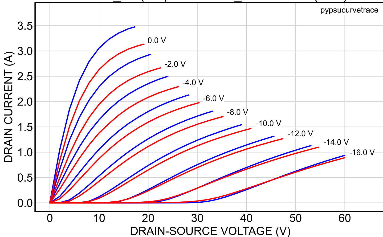
2SK82_49 (red) vs. 2SK82_52reserved (blue)
