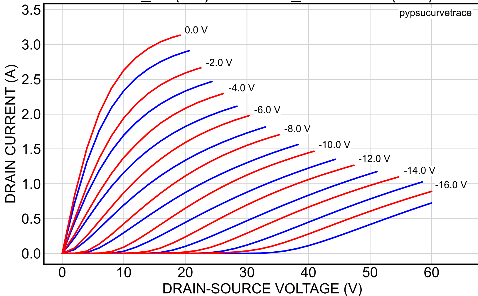
2SK82_49 (red) vs. 2SK82_56reserved (blue)
