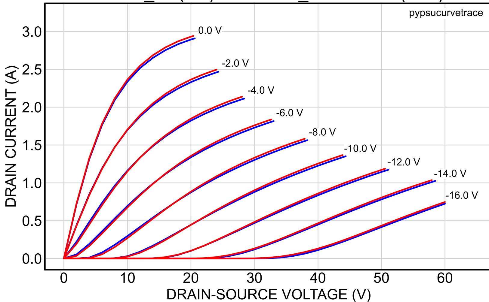
2SK82_50 (red) vs. 2SK82_56reserved (blue)
