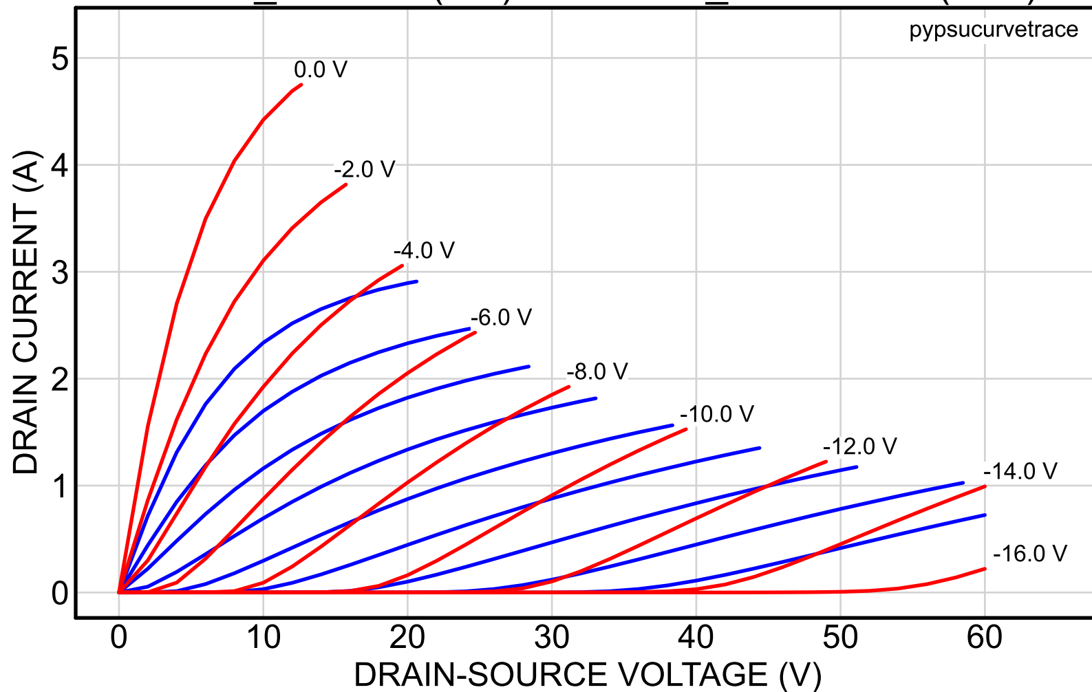
2SK82_51NAbb (red) vs. 2SK82_56reserved (blue)
