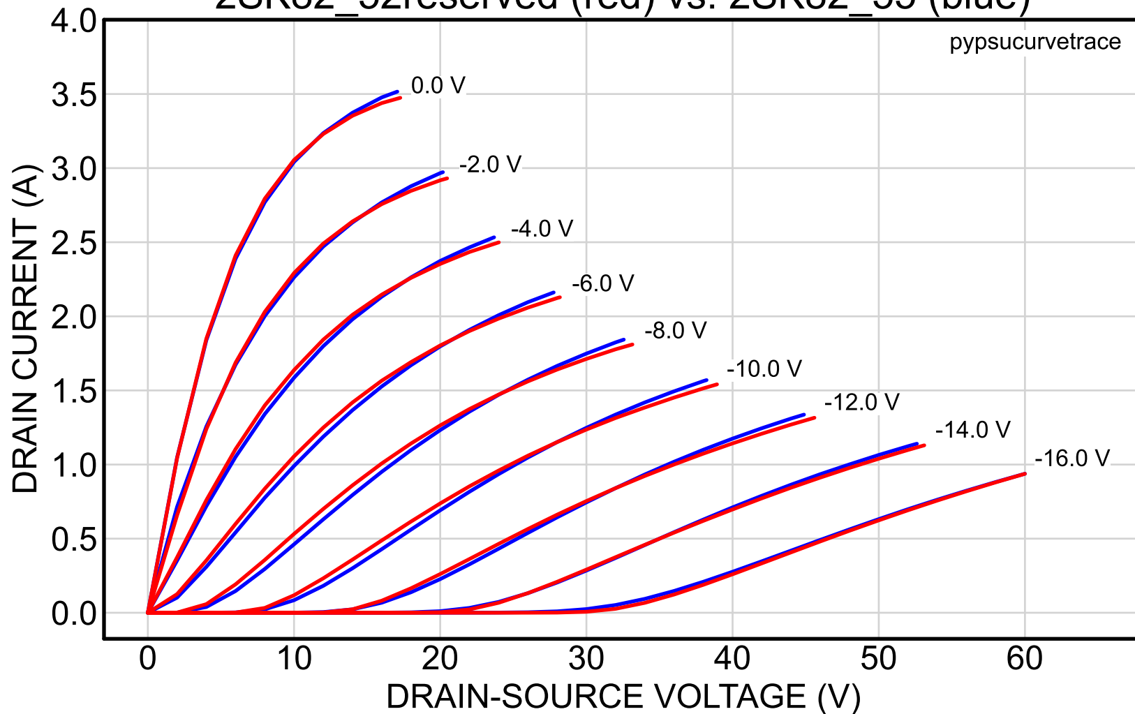
2SK82_52reserved (red) vs. 2SK82_55 (blue)
