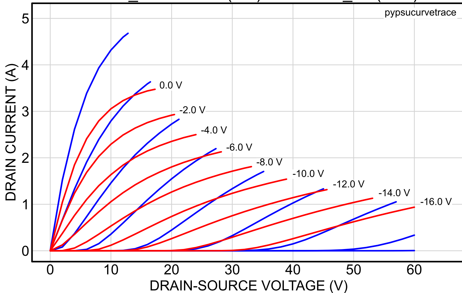
2SK82_52reserved (red) vs. 2SK82_57 (blue)
