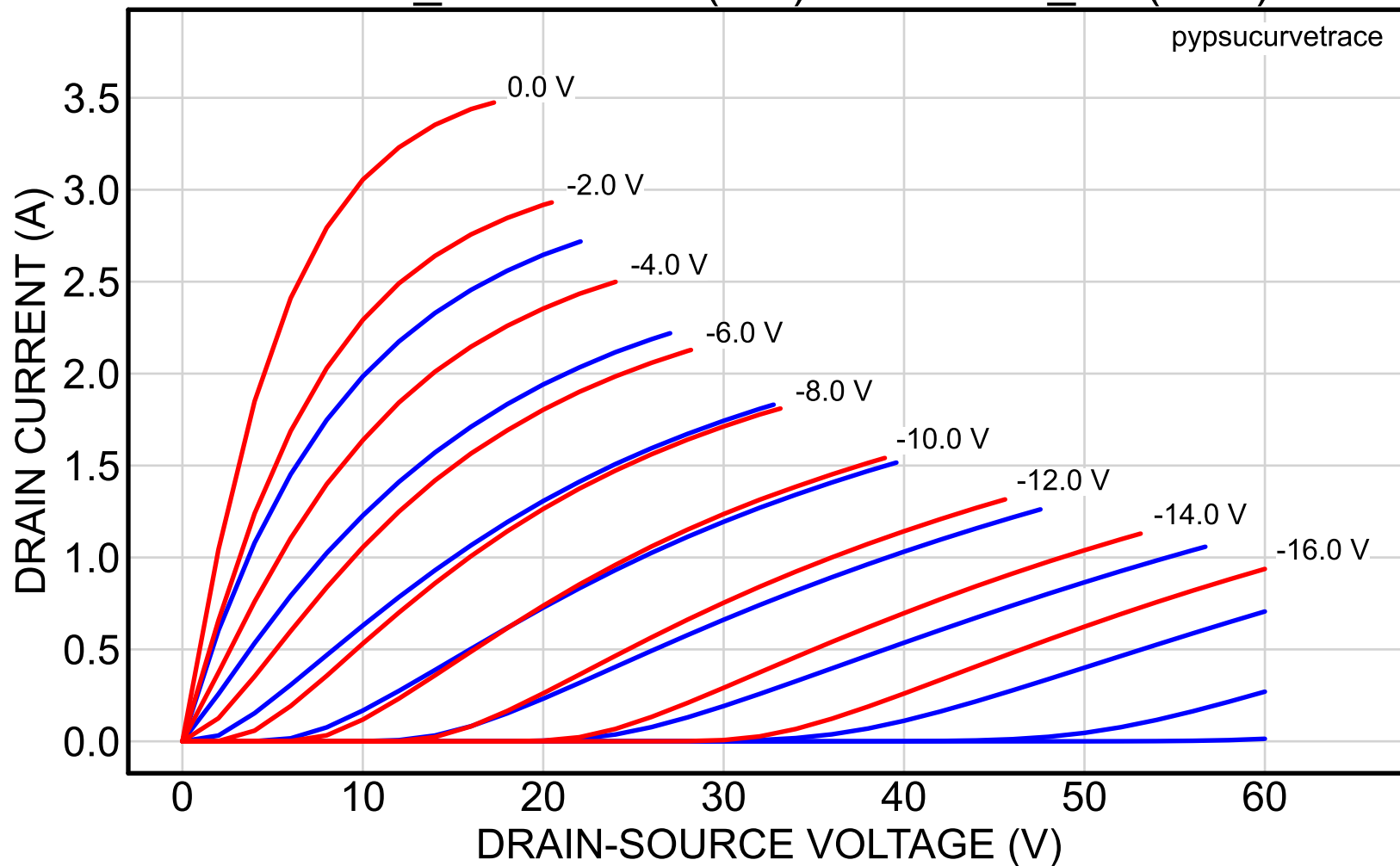
2SK82_52reserved (red) vs. 2SK82_58 (blue)
