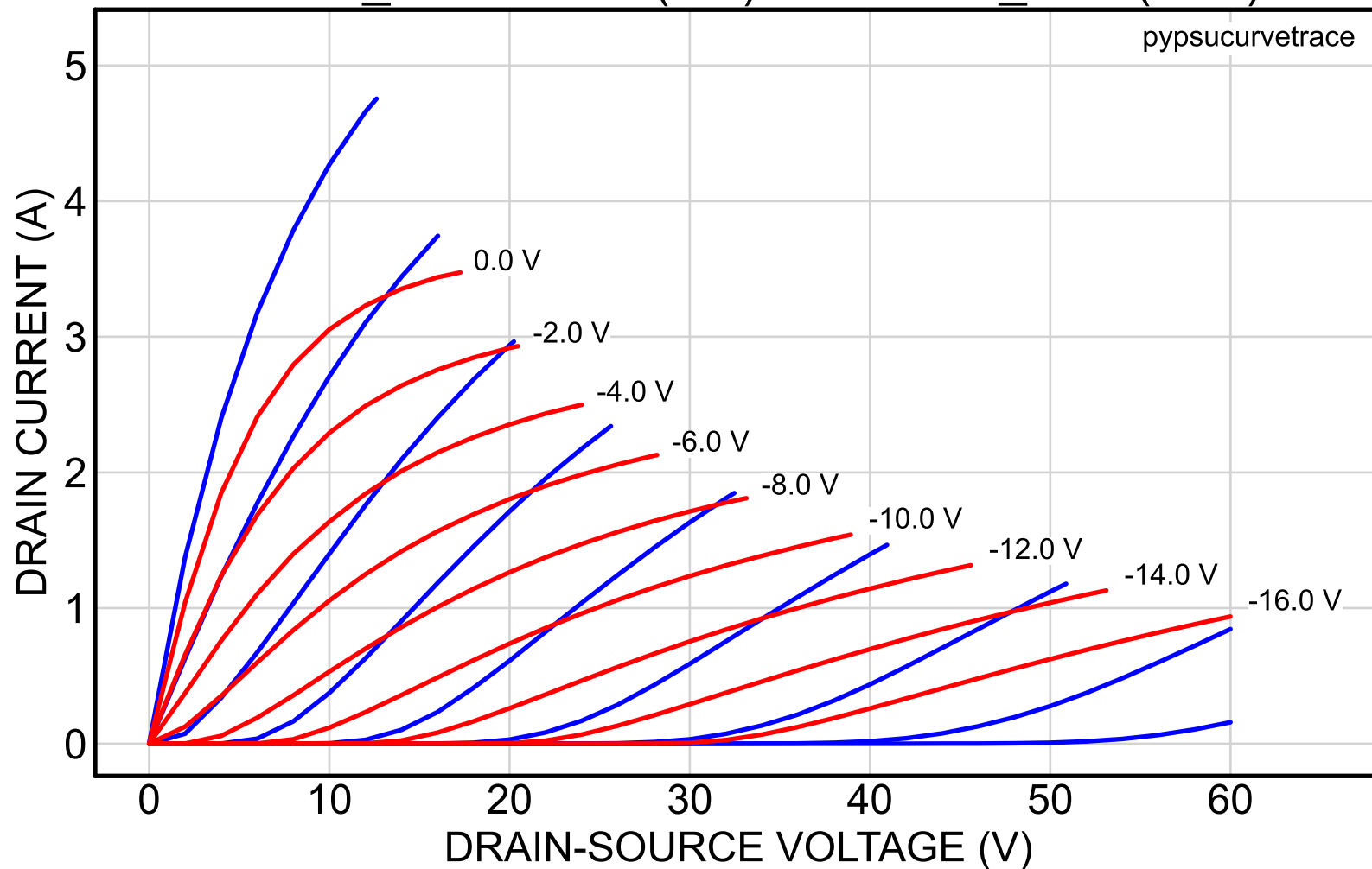
2SK82_52reserved (red) vs. 2SK82_5NA (blue)
