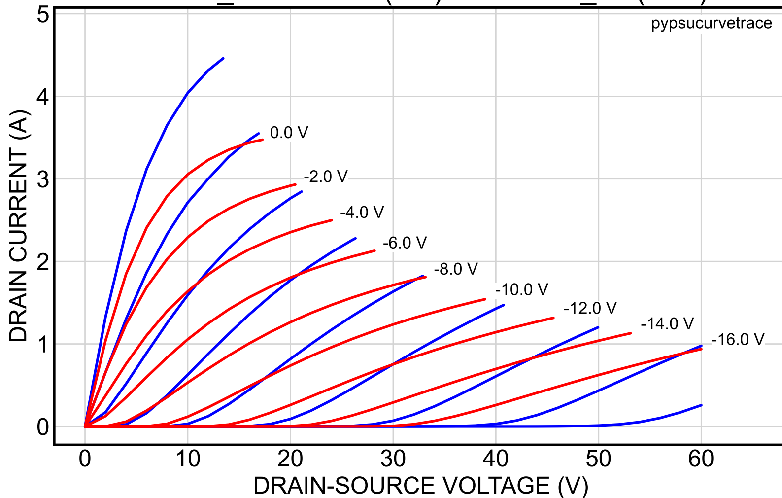
2SK82_52reserved (red) vs. 2SK82_60 (blue)
