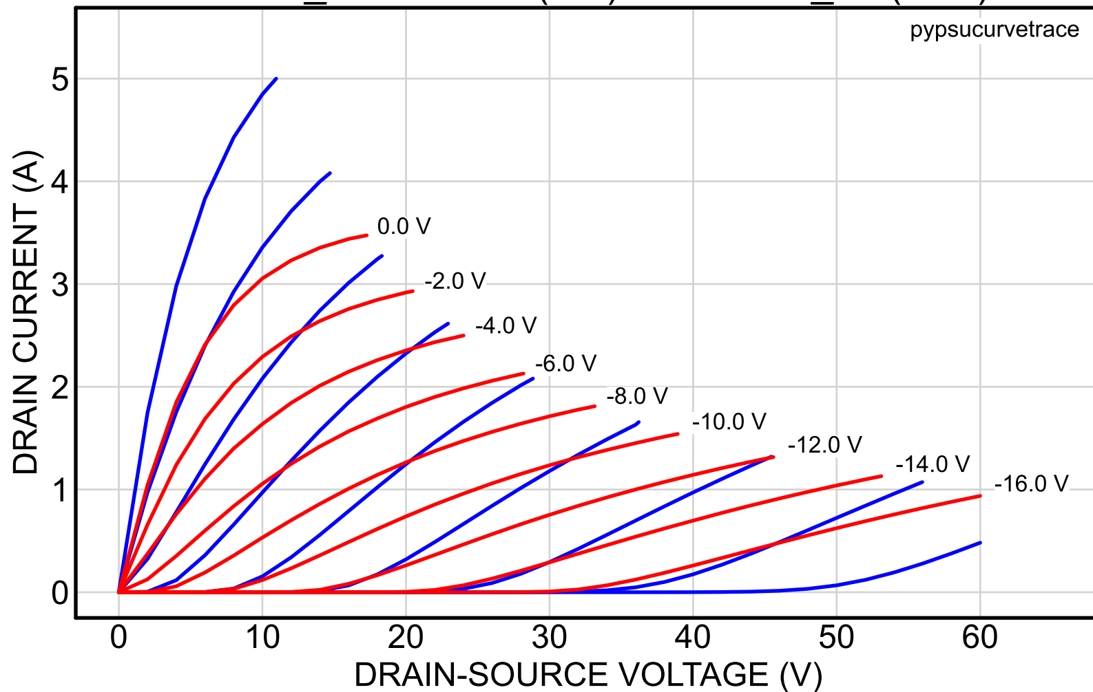
2SK82_52reserved (red) vs. 2SK82_61 (blue)
