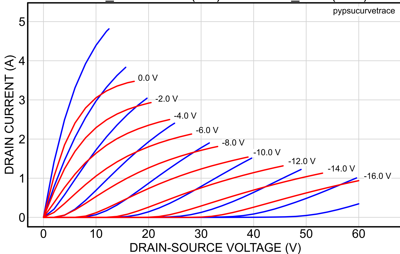
2SK82_52reserved (red) vs. 2SK82_6NA (blue)
