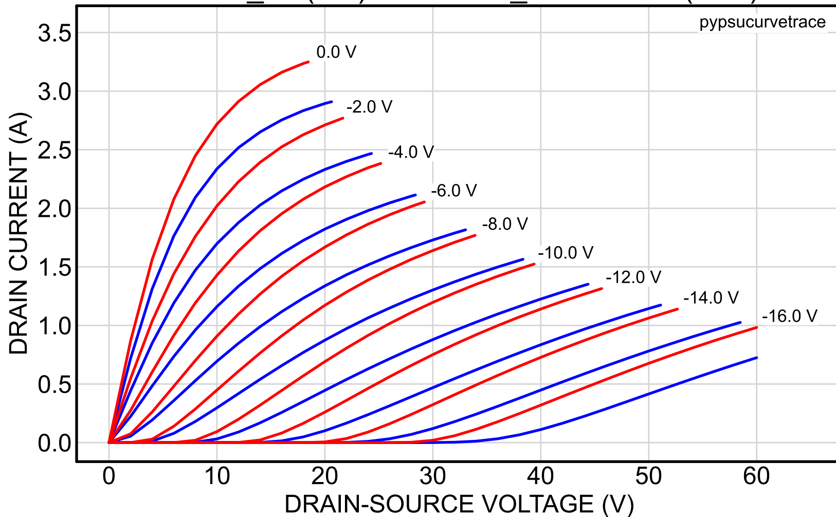
2SK82_53 (red) vs. 2SK82_56reserved (blue)
