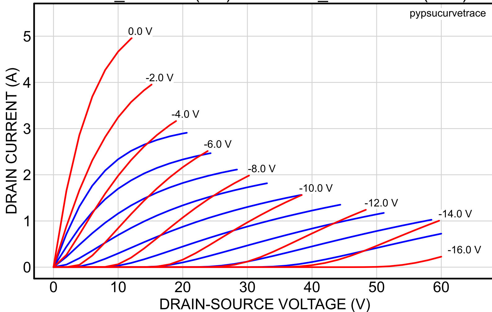
2SK82_54NAbb (red) vs. 2SK82_56reserved (blue)
