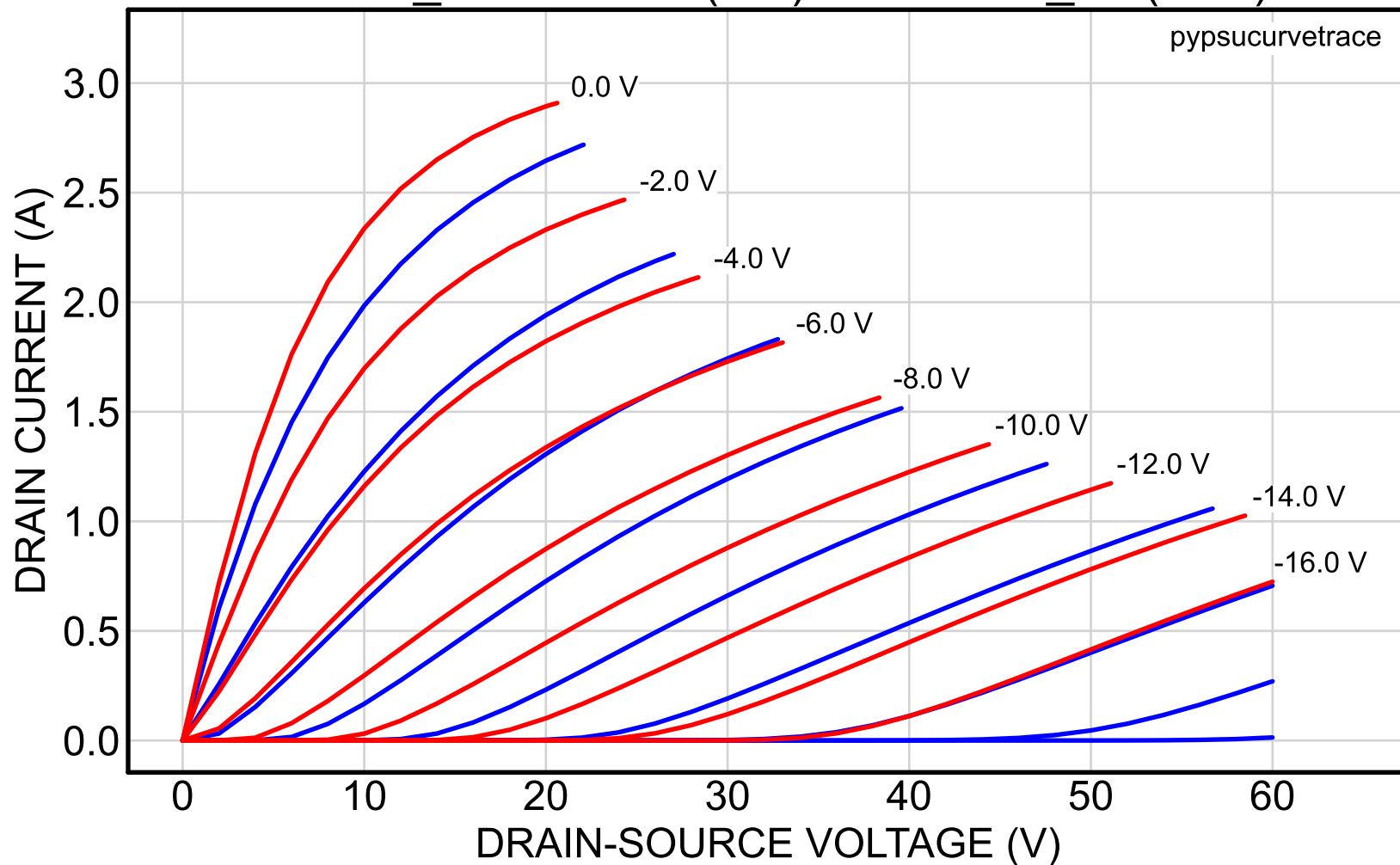
2SK82_56reserved (red) vs. 2SK82_58 (blue)
