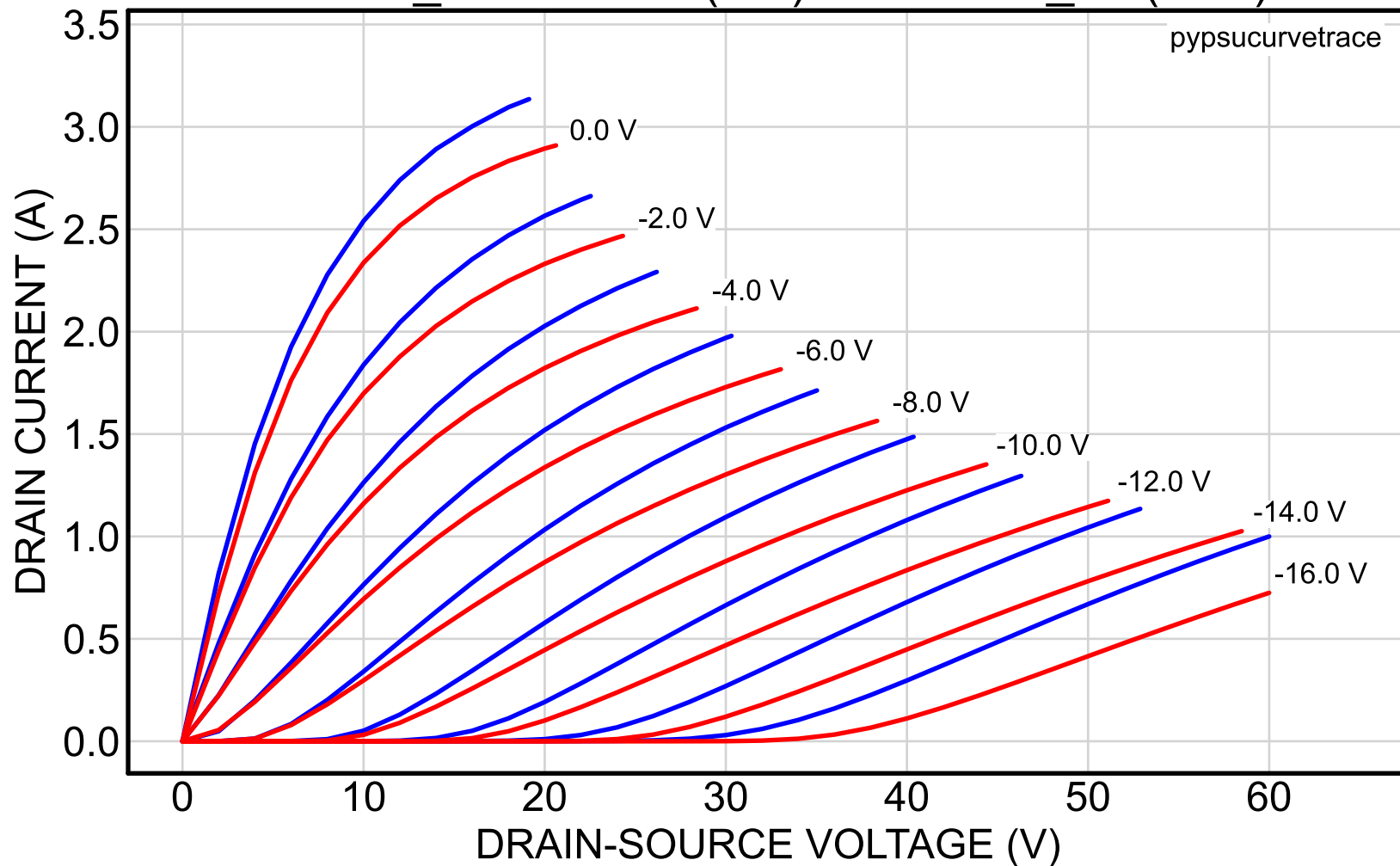
2SK82_56reserved (red) vs. 2SK82_59 (blue)
