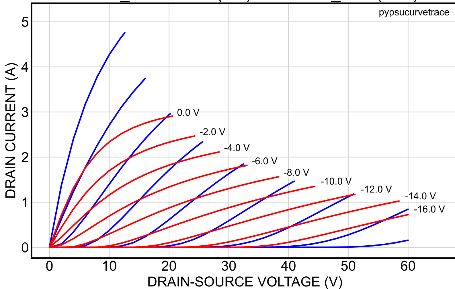
2SK82_56reserved (red) vs. 2SK82_5NA (blue)
