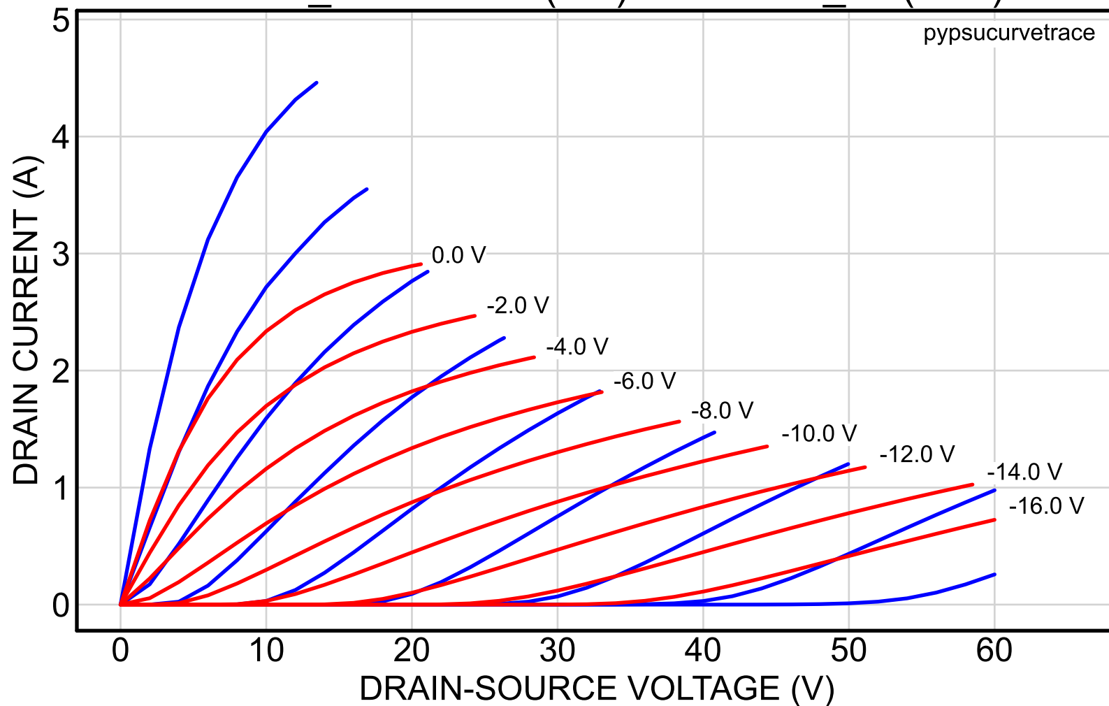
2SK82_56reserved (red) vs. 2SK82_60 (blue)
