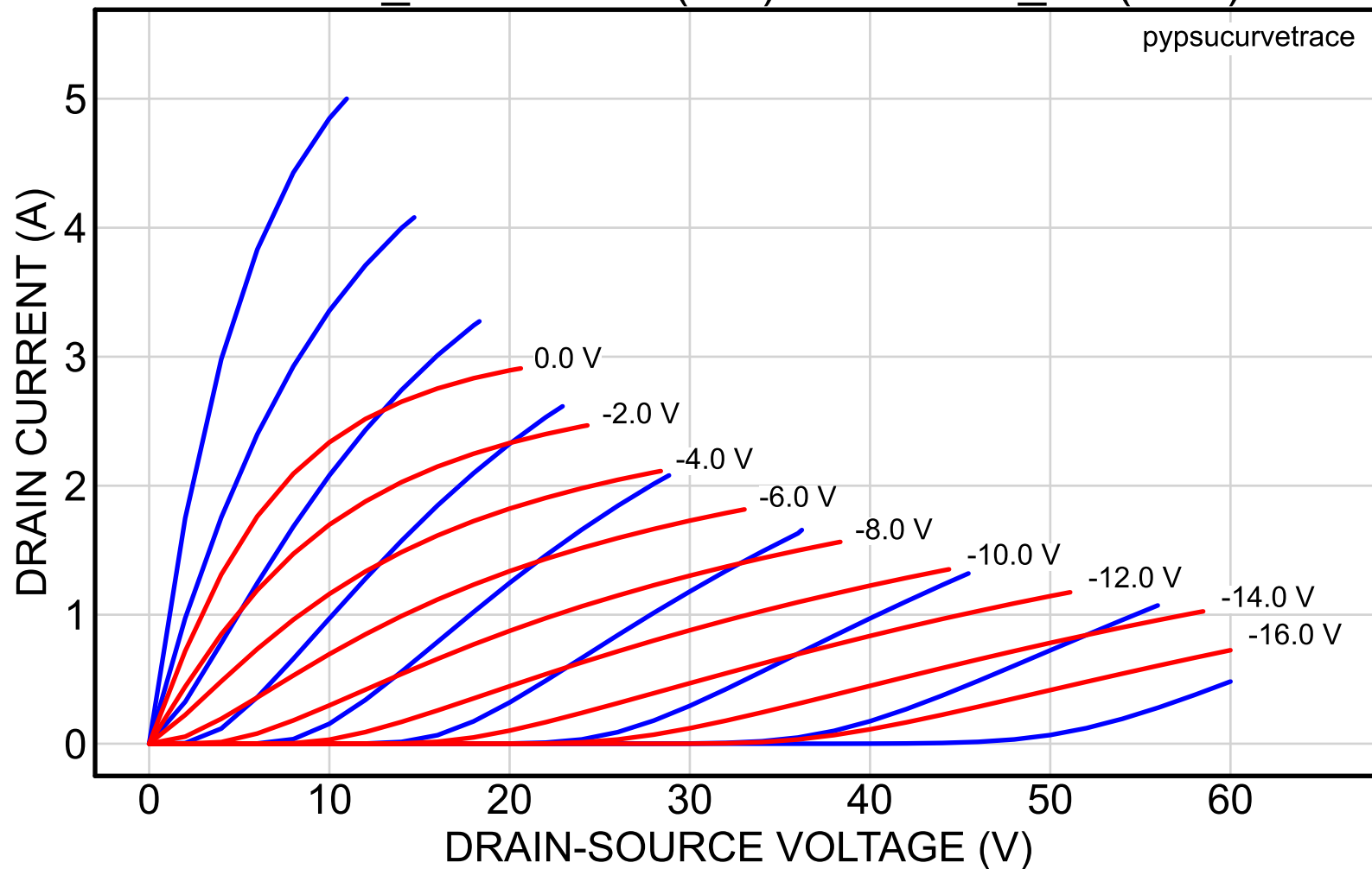
2SK82_56reserved (red) vs. 2SK82_61 (blue)
