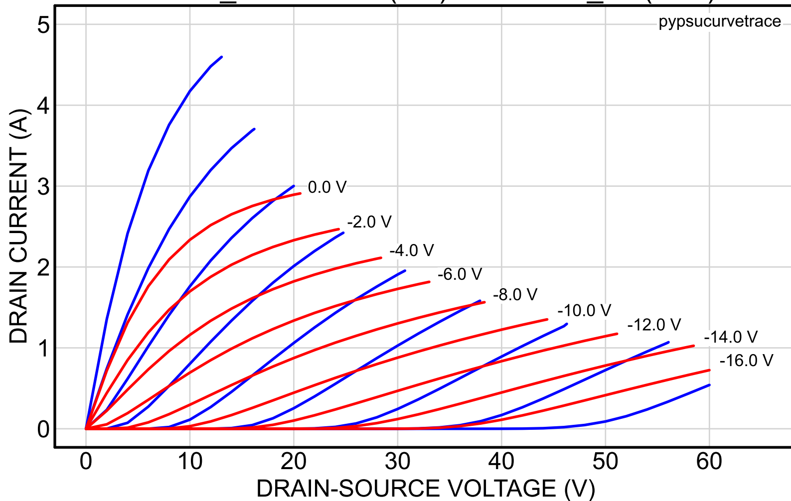
2SK82_56reserved (red) vs. 2SK82_62 (blue)
