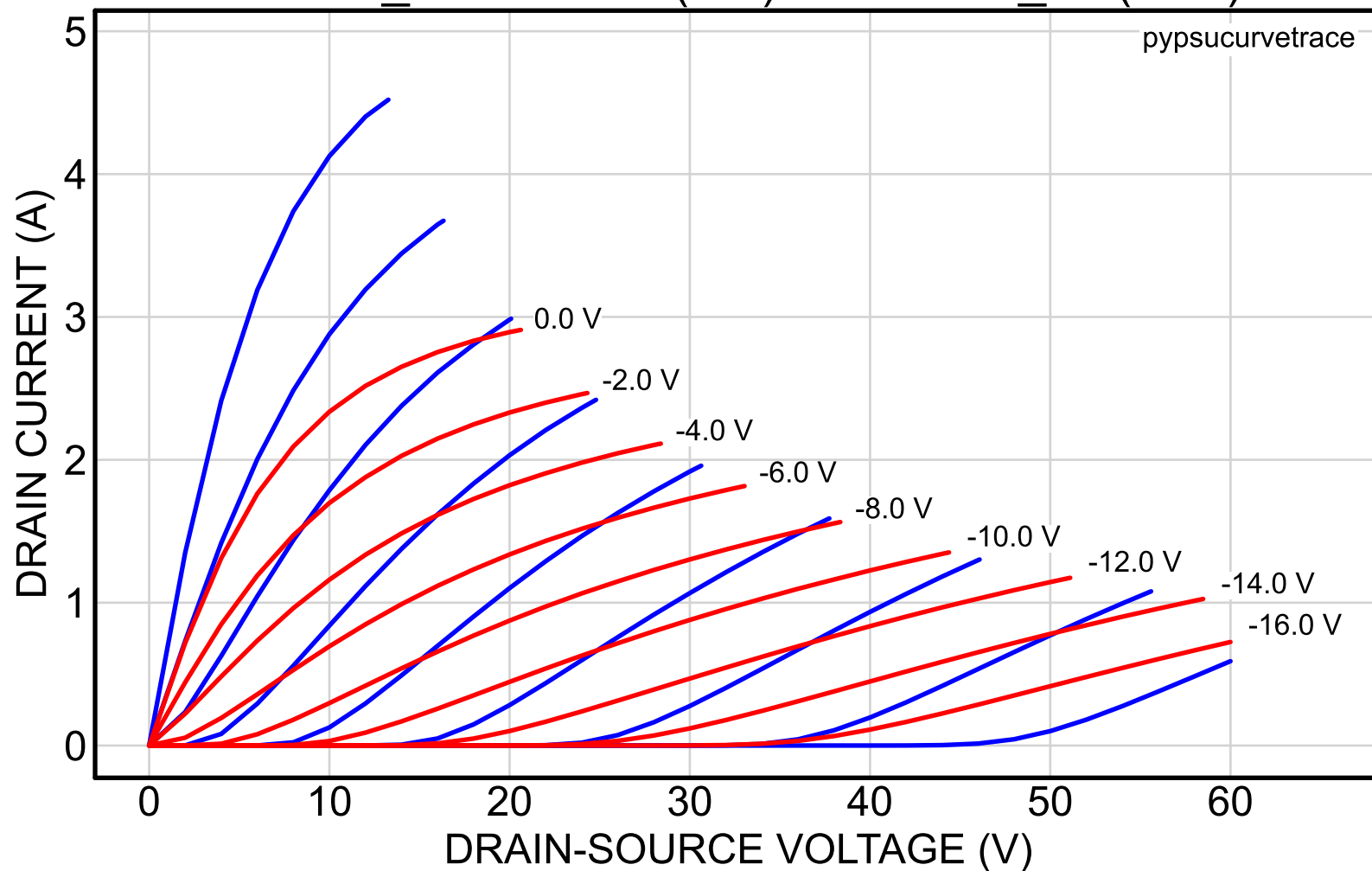
2SK82_56reserved (red) vs. 2SK82_63 (blue)
