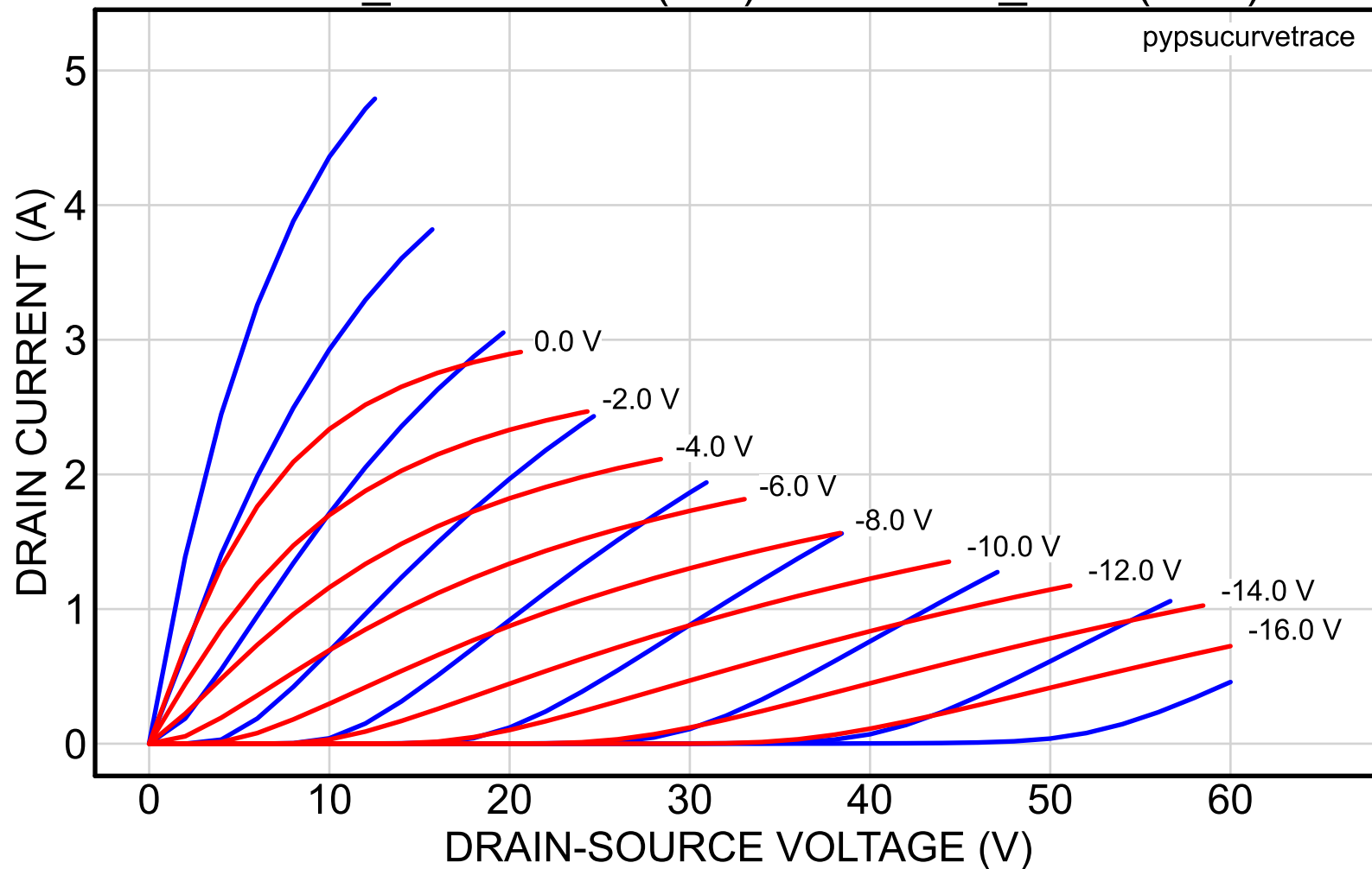
2SK82_56reserved (red) vs. 2SK82_8NA (blue)
