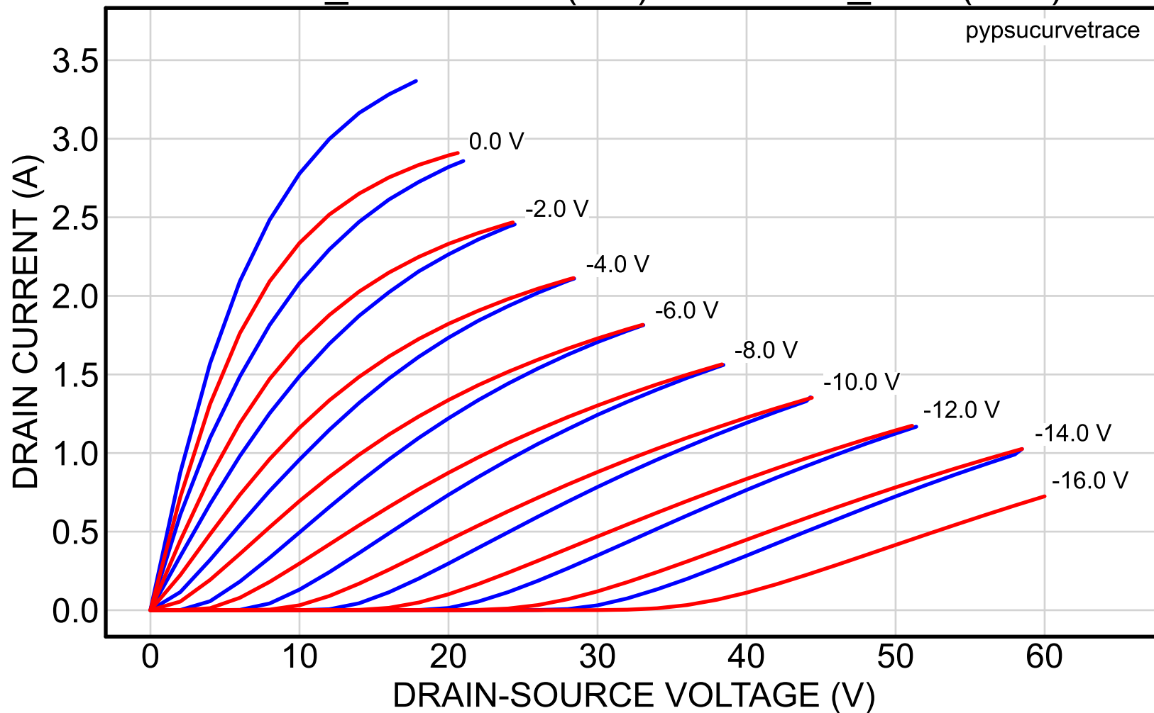
2SK82_56reserved (red) vs. 2SK82_9NA (blue)
