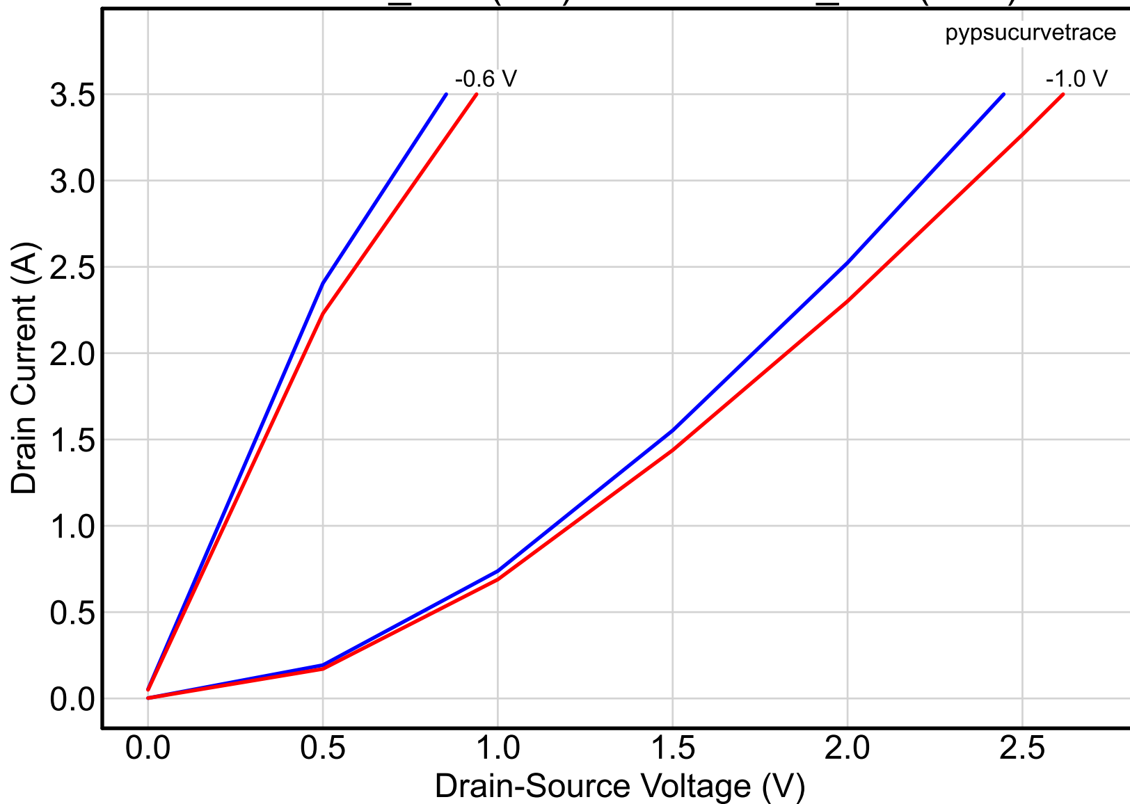
LD1014D_250 (red) vs. LD1014D_340 (blue)
