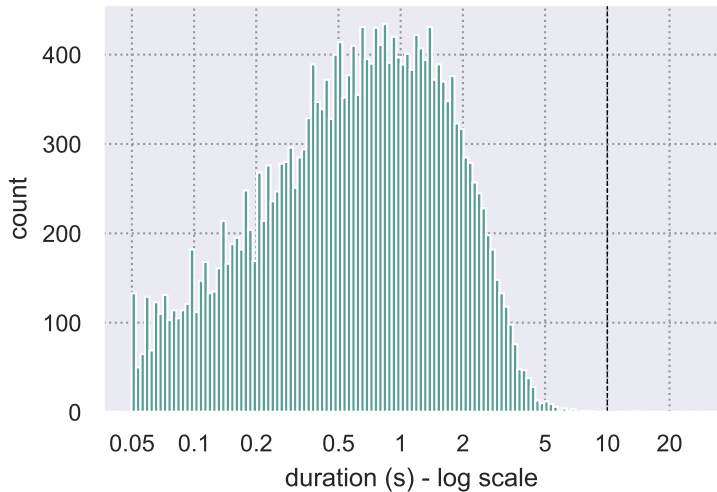
Distribution of response duration group EXP20
