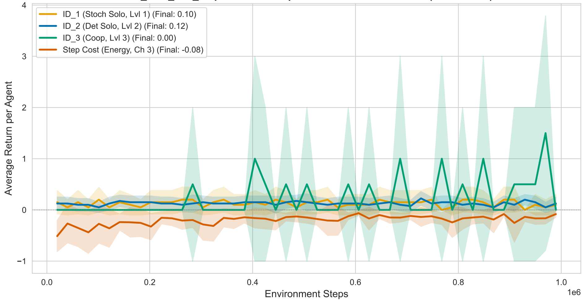
Run_max_adv_stepcost - Decomposed Channel Breakdown (4 Channels)
