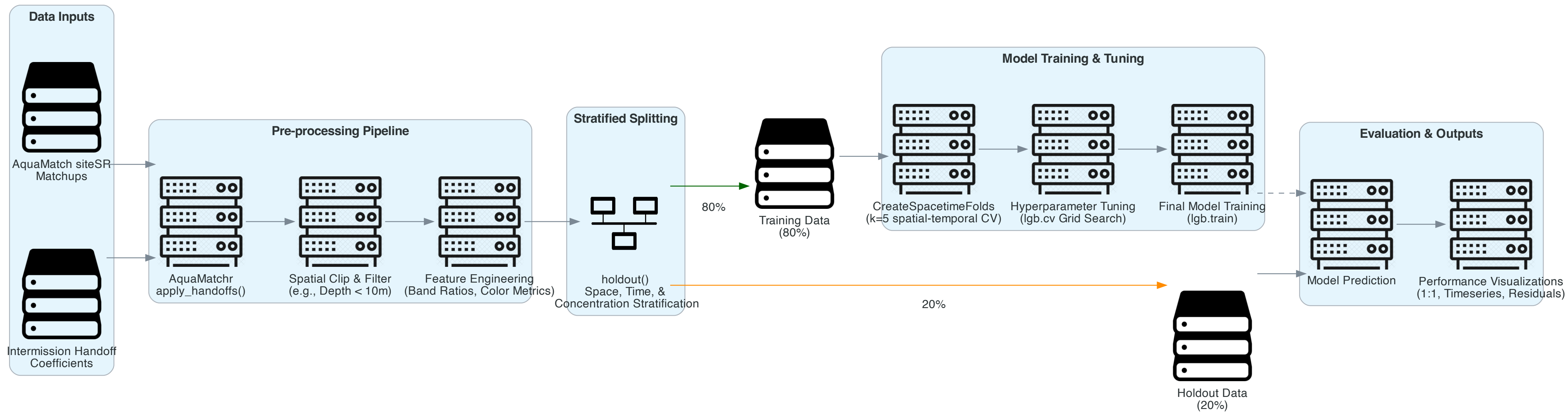
AquaSat V2 LightGBM Modeling Workflow
