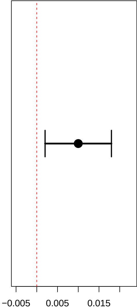
Frequentist: Effect Size and 95% C
