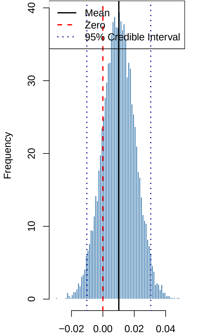
Bayesian: Posterior Distribution of L
