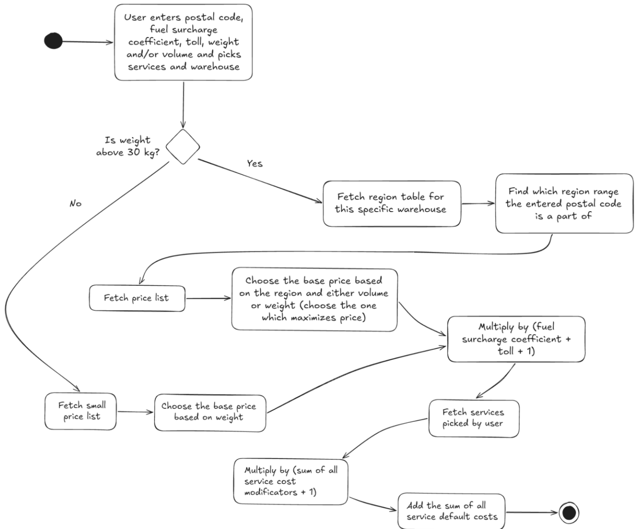
Figure 6. Activity diagram - shipment cost estimation
