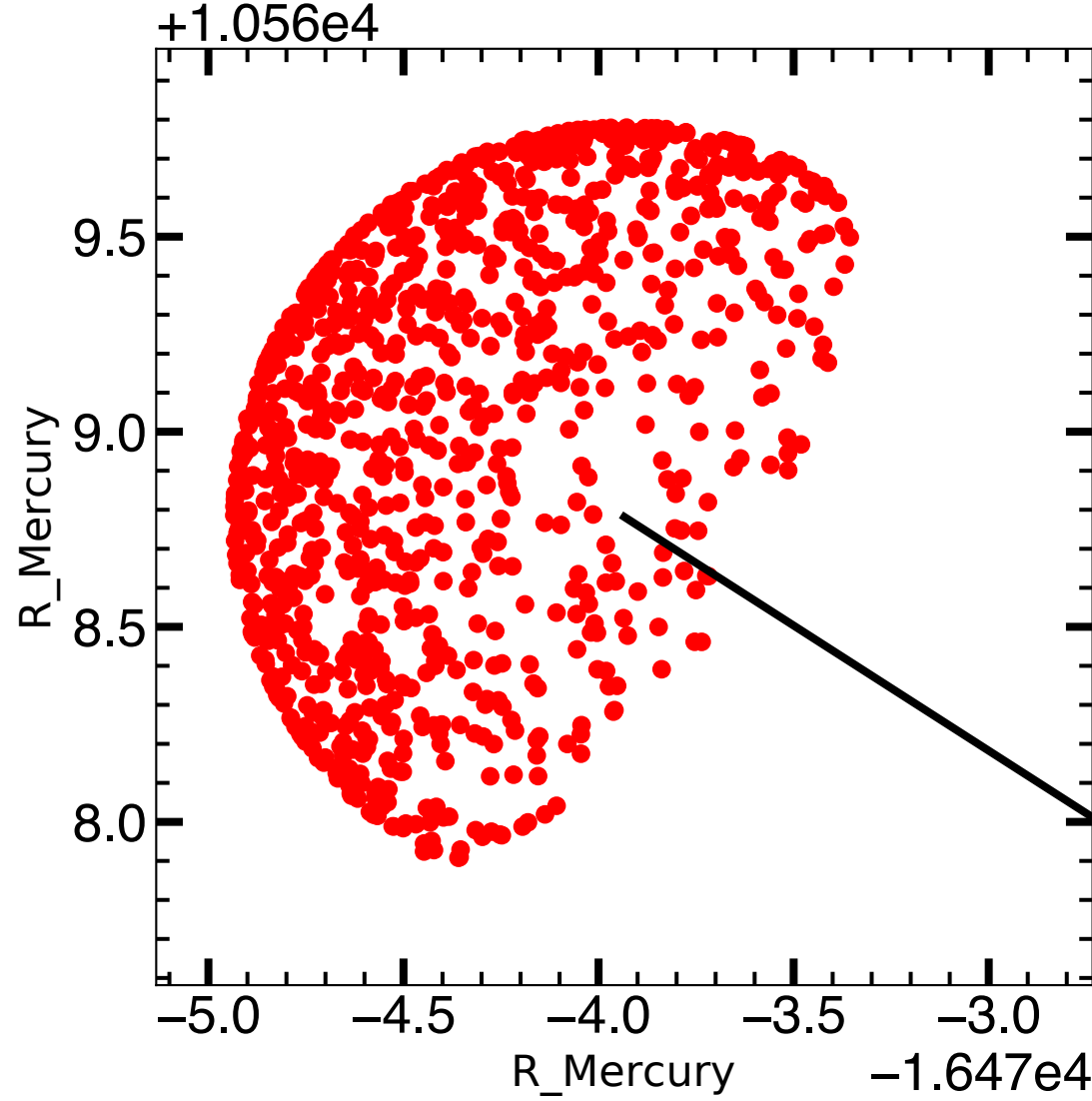
Starting Point, frame=MERCURYSOLAR
