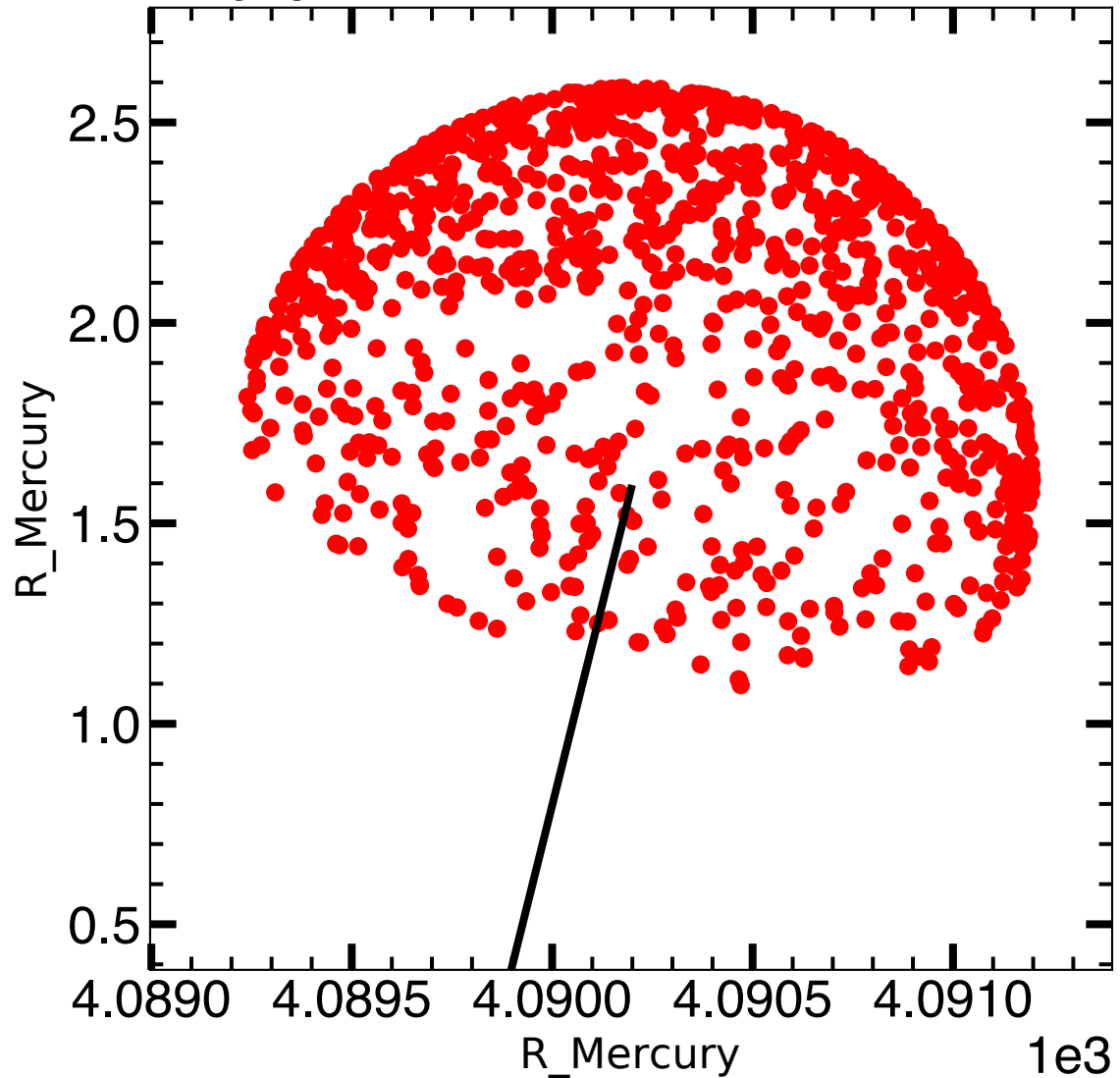
+1.64e4 Initial State, frame=J2000
