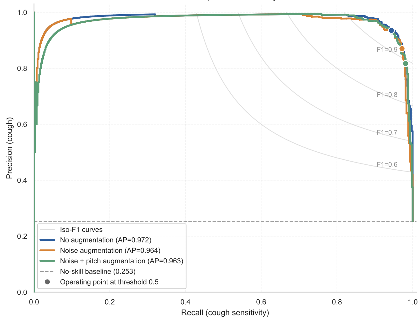
Precision–recall comparison on the Stage 1 test set
