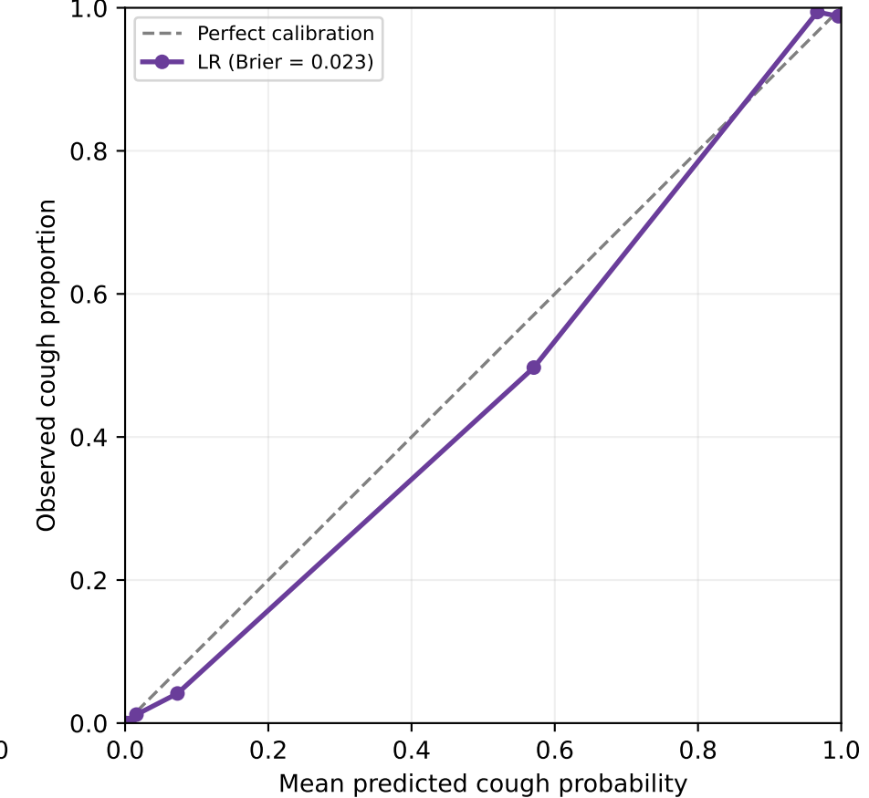
(c) Calibration curve
