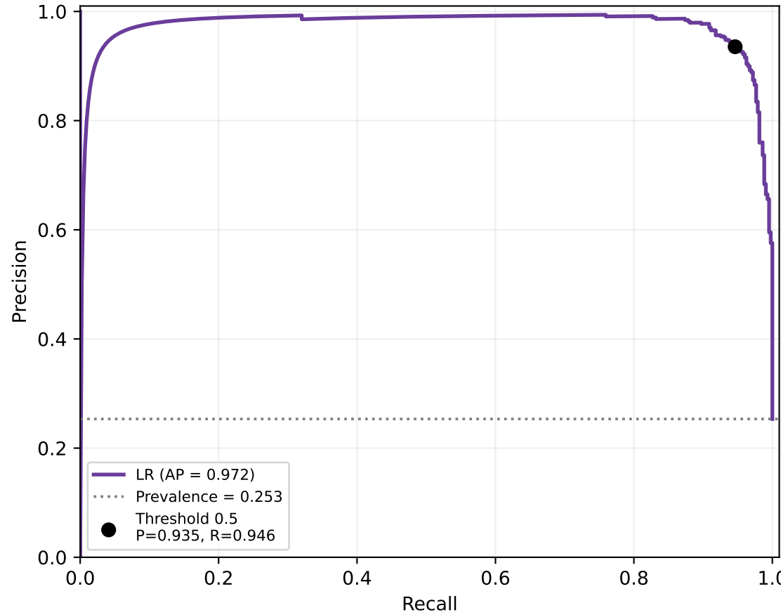
(b) Precision-recall curve
