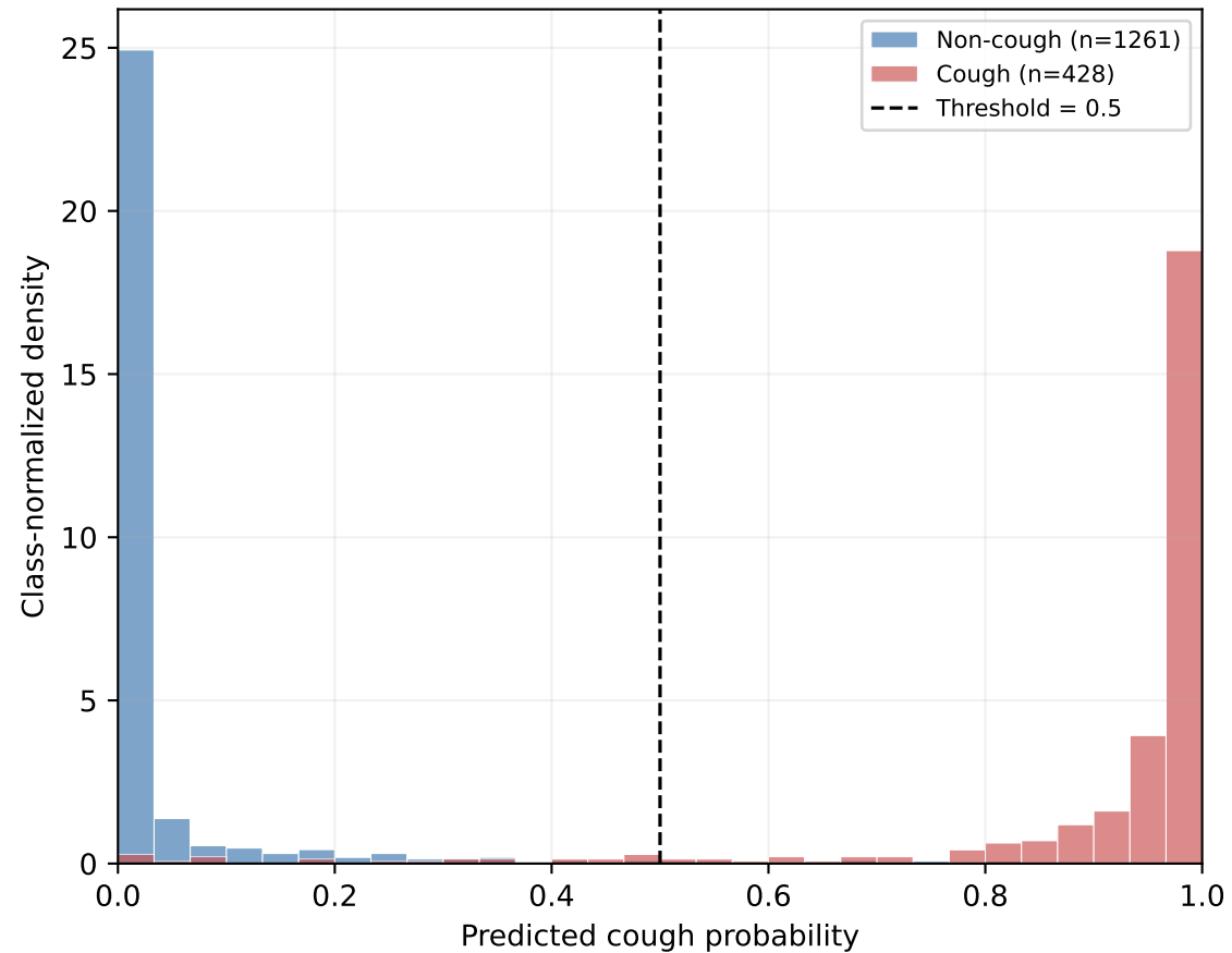
(a) Probability distribution
