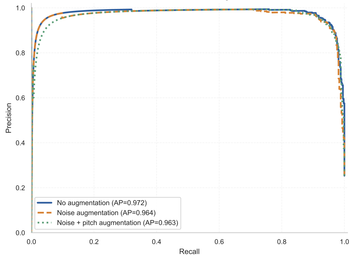
Precision–recall curves on the Stage 1 test set
