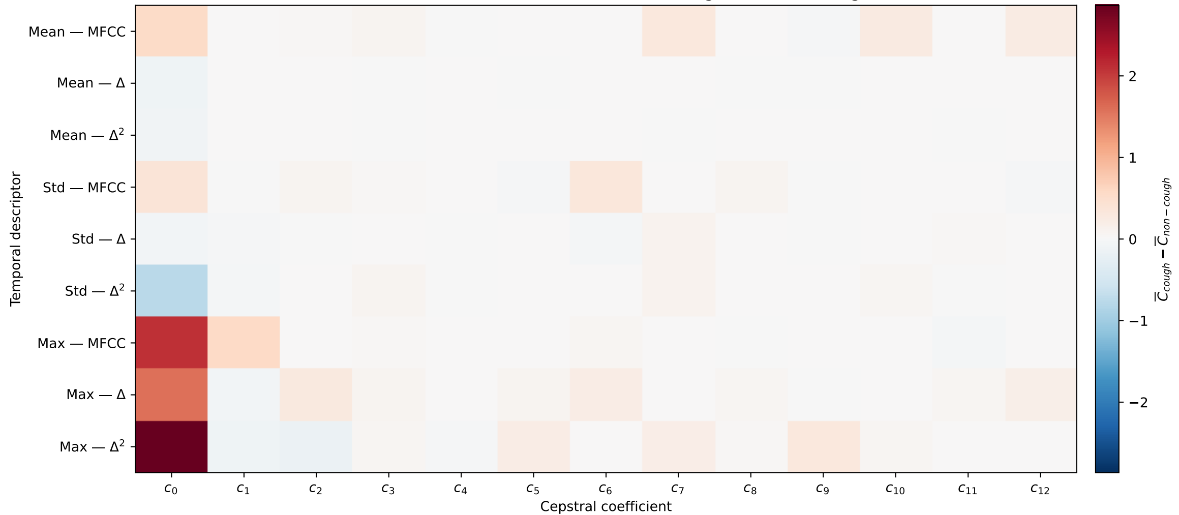
Difference in mean feature contribution: cough minus non-cough
