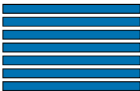
2020 embedding (64-D)
