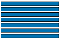
2018 embedding (64-D)
