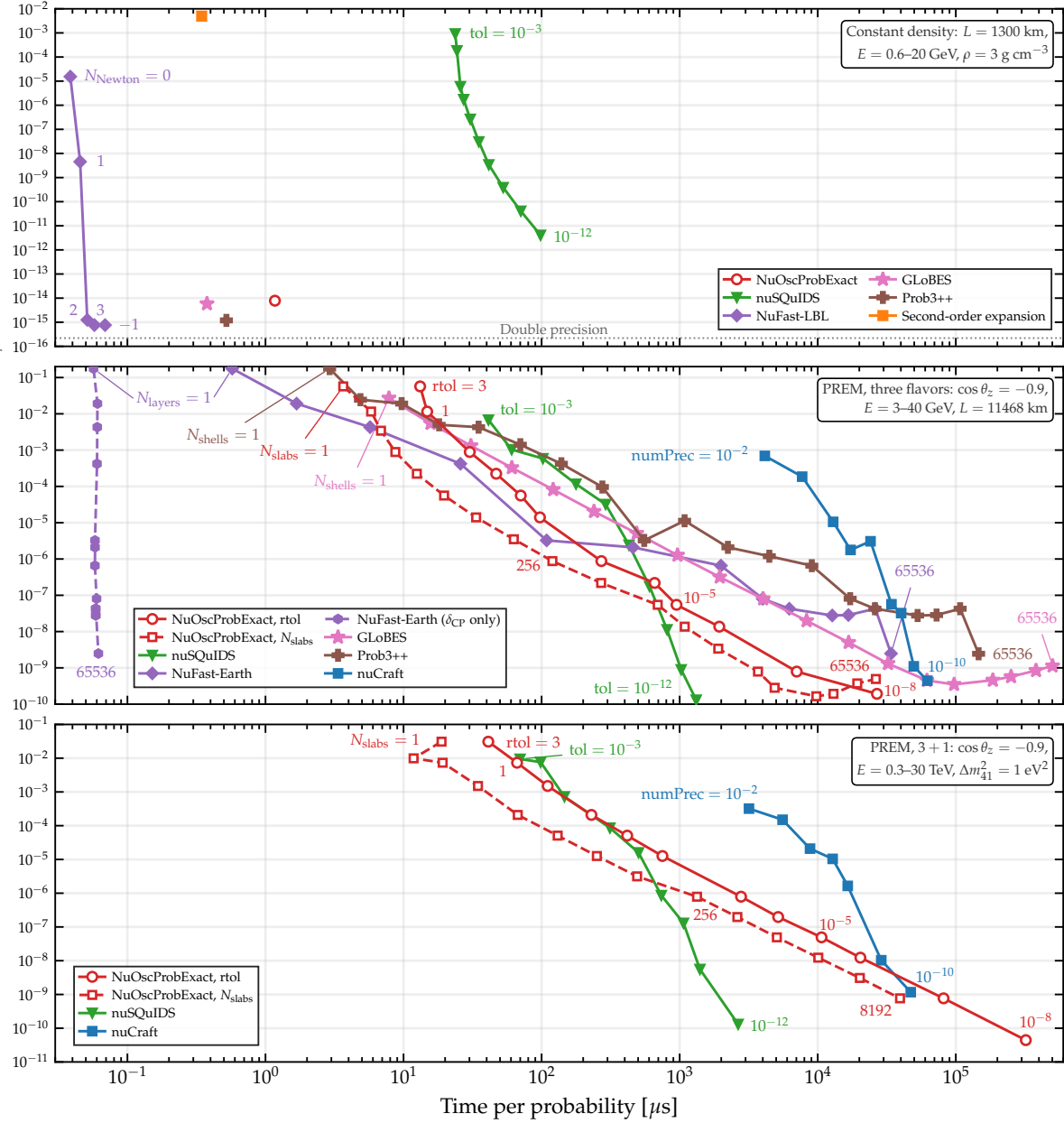
Error vs. a 50-digit converged solution, \max_a |\Delta P_{\nu_\mu \rightarrow \nu_a}|
