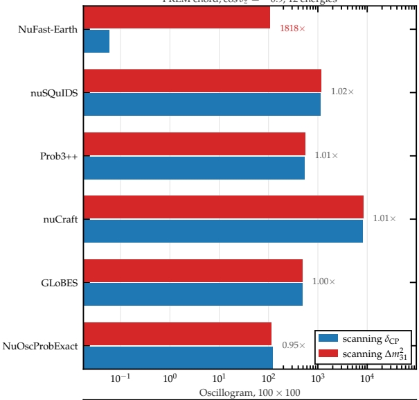
PREM chord, \cos \theta_z = -0.9 , 12 energies
