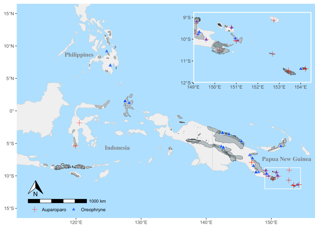
Figure 3: The known distribution of Oreophryne sensu lato is plotted in grey polygons (data source IUCN 2025), with points indicating Auparoparo (red) and Oreophryne (blue) as identified by our phylogeny Figure 2. Note that there is overlap among points
