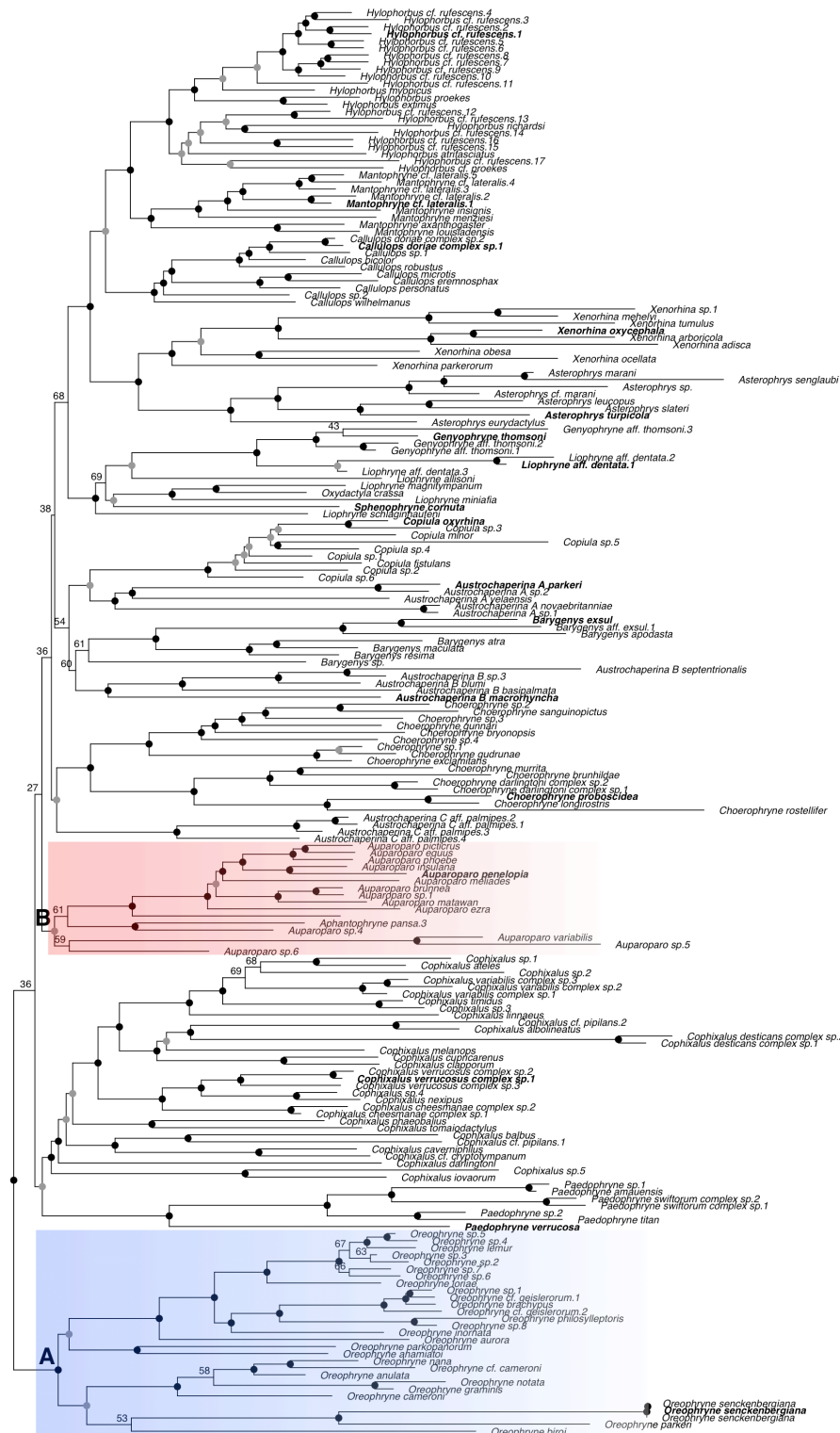
Figure 2: Molecular phylogenetic hypothesis of Asterophrinae showing polyphyly of Oreophryne sensu lato, into two reciprocally monophyletic clades, node A is Oreophryne (blue clad) and node B is Auparoparo (red clad) based on the position of the type species Oreophryne senckenbergiana . Molecular evidence includes two mitochondrial and three nuclear markers analyzed using Maximum Likelihood following Rivera et al. (2017); Hill et al. (2022). Nodal support: black dots indicate ML bootstrap support \geq 95\% , grey dots \geq 75\% , numeric values given for nodes below 75% support. Outgroup taxa excluded.
