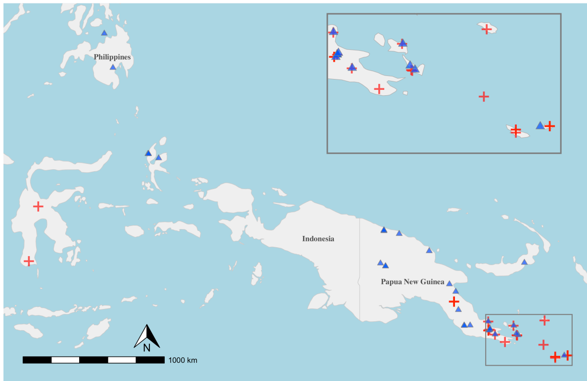
Figure 3: Distributions of and Auparoparo (red) and Oreophryne (blue).
