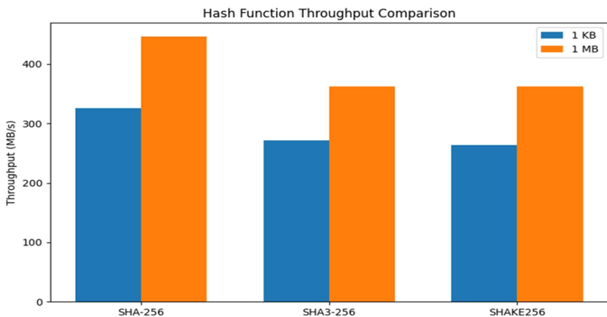
Figure V.3: Hash function throughput (MB/s) at 1 KB and 1 MB input sizes. SHA-256 outperforms SHA3-256 and SHAKE256 by approximately 19% at 1 MB due to hardware SHA-NI acceleration.
