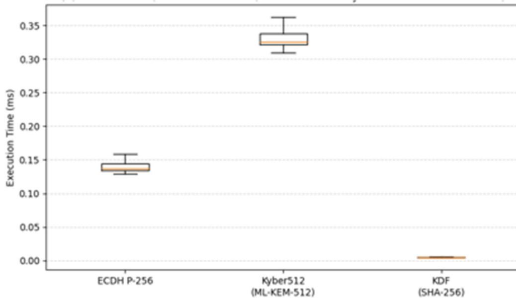
Figure V.6: Box plot comparing the latency distribution (ms) of each component in the hybrid ECDH + ML-KEM-512 key establishment workflow. The figure shows that ML-KEM-512 and ECDH P-256 account for the majority of total hybrid latency, while the SHA-256 KDF contributes less than 1% of the total overhead
