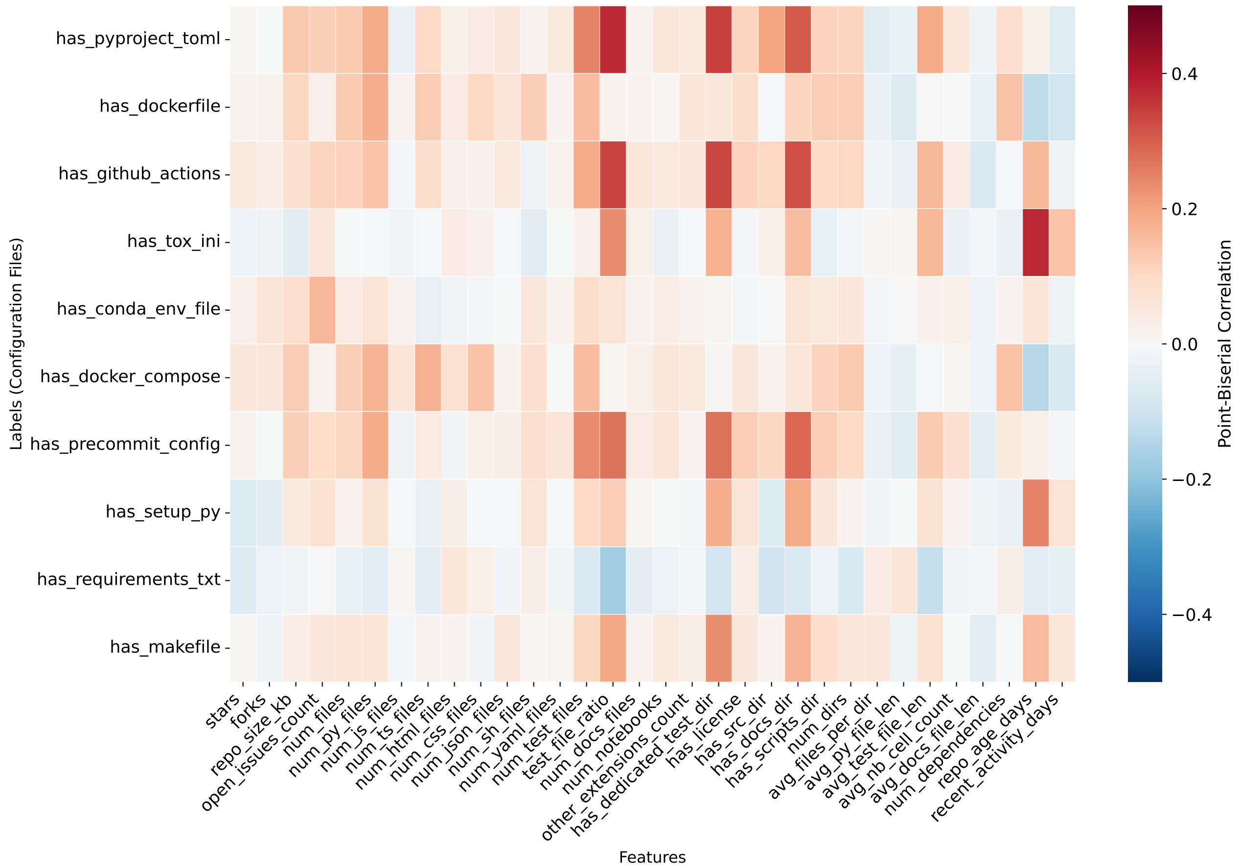
Feature-Label Correlation Matrix
