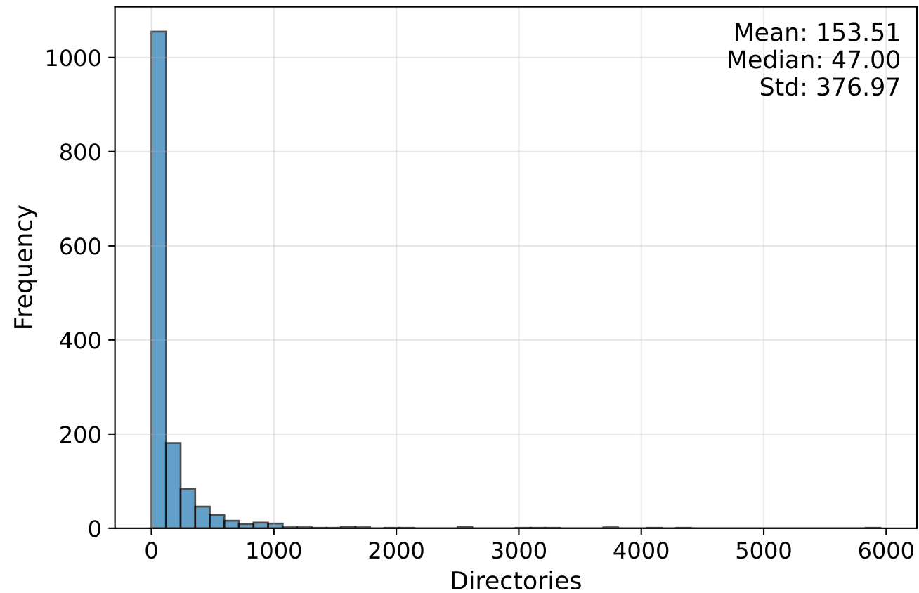
Directories Distribution
