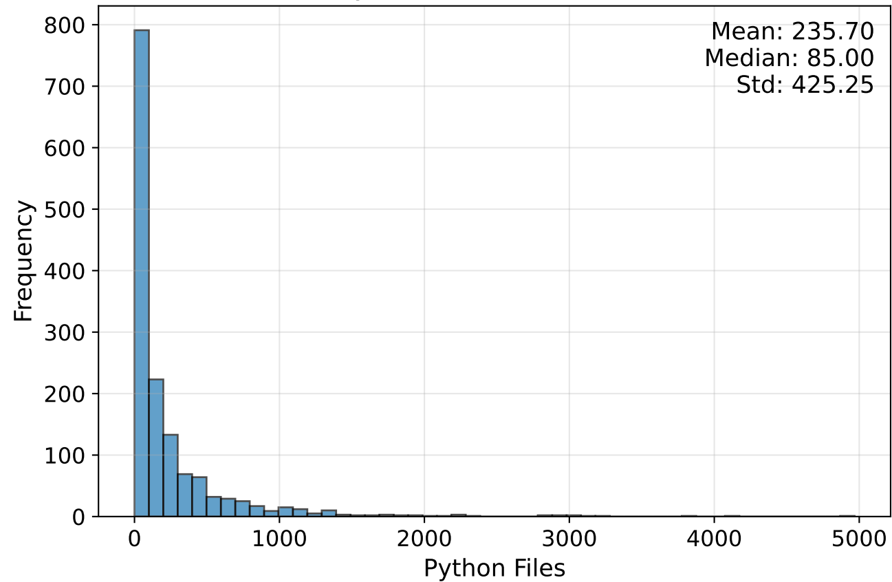
Python Files Distribution
