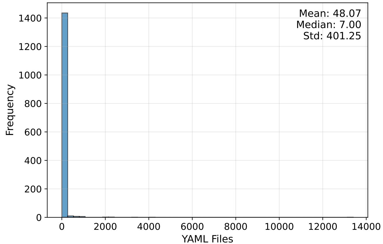
YAML Files Distribution
