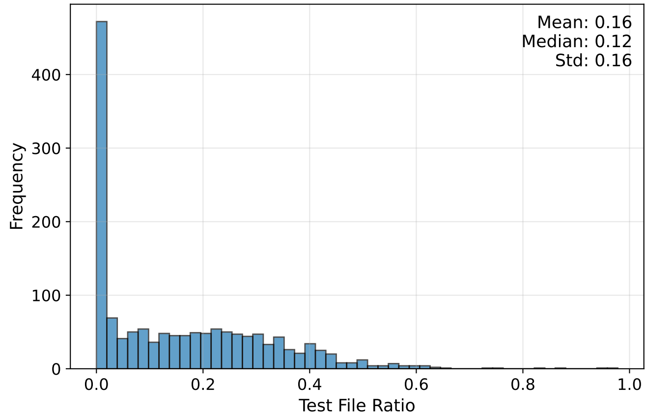
Test File Ratio Distribution
