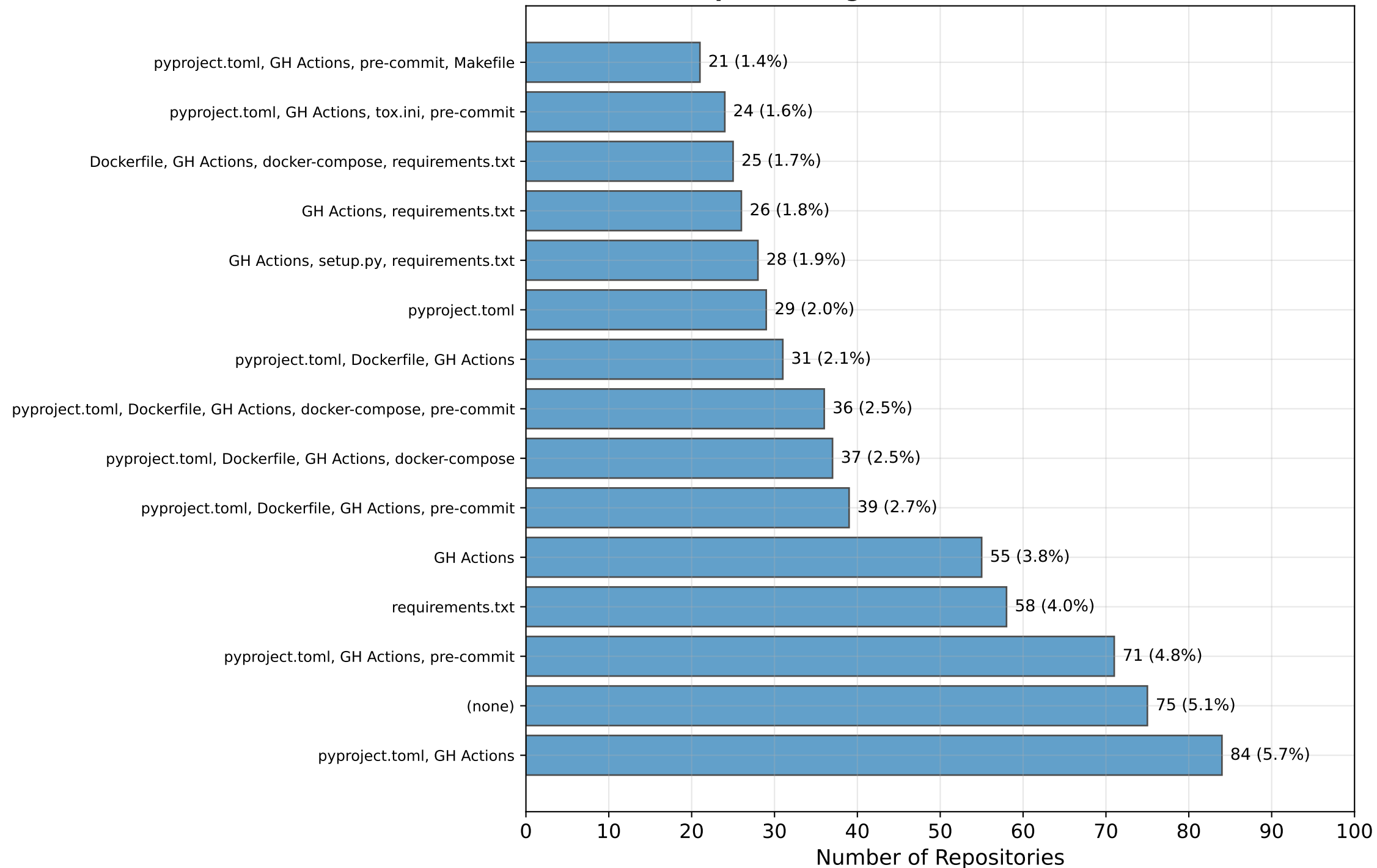
Top 15 Configuration File Combinations
