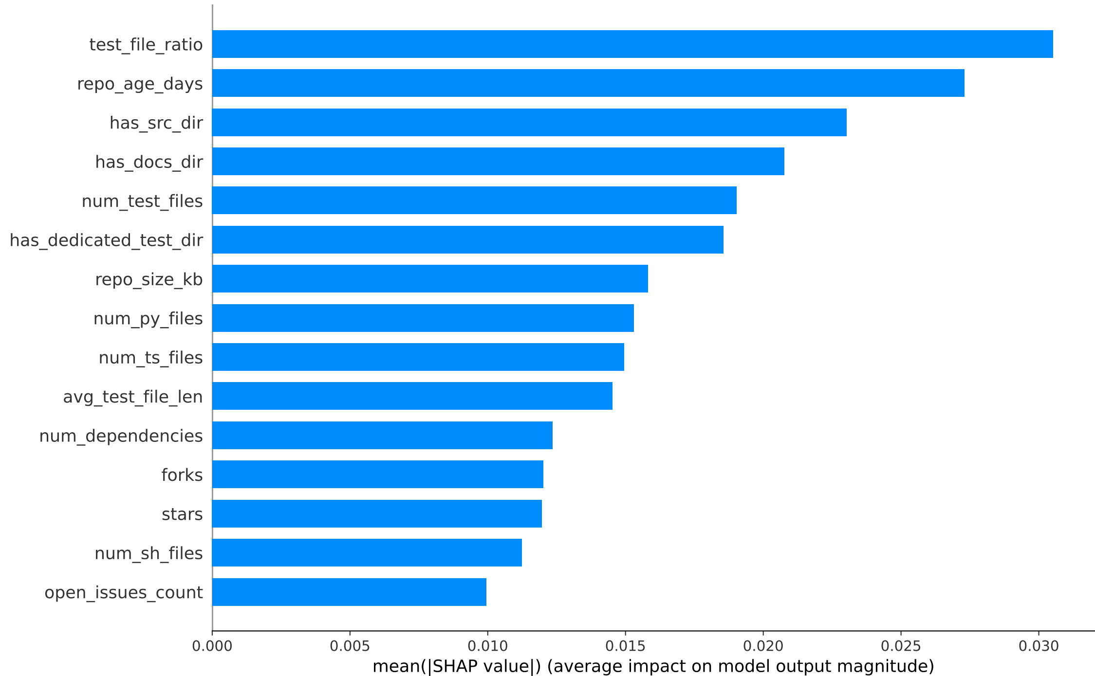
SHAP Mean Absolute Impact (neural_network)
